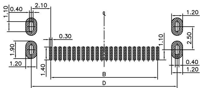
RECOMMENDED PCB PATTERN DIM. TOLERANCE : ±0.05
