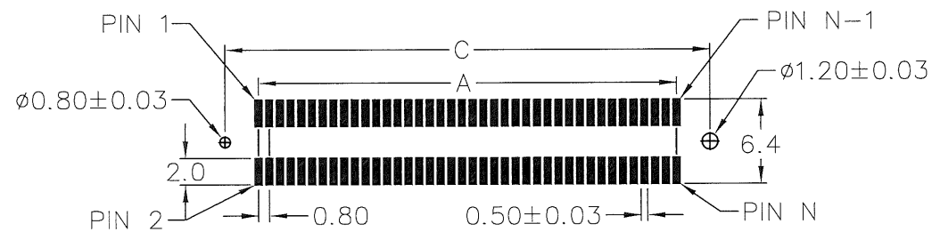
RECOMMENDED PCB LAYOUT (PCB TOLERANCE ±0.05)
